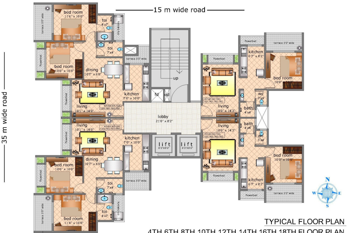
4TH,6TH,8TH,10TH,12TH,14TH,16TH,18TH FLOOR PLAN
